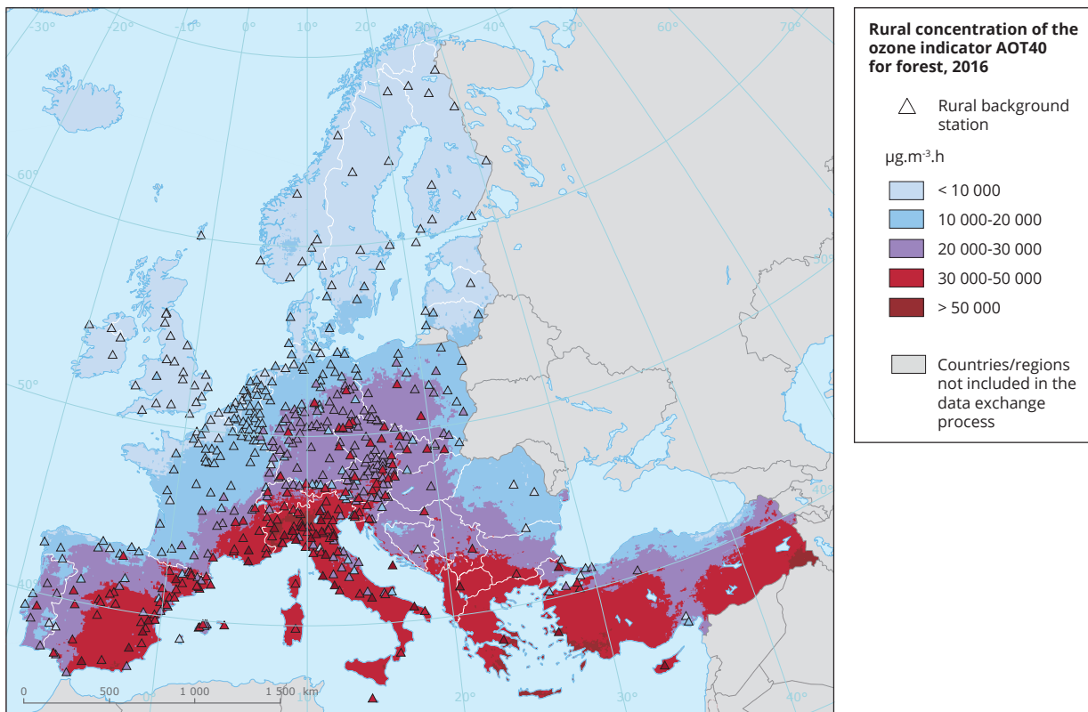
Map 11.2 Rural concentration of the O 3 indicator AOT40 for forests, 2016
